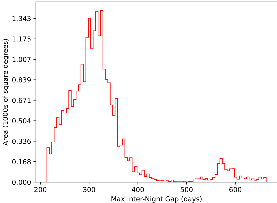
ddf_loaded_half_fl15_v3.4_10yrs All sky i band: Max Inter-Night Gap
