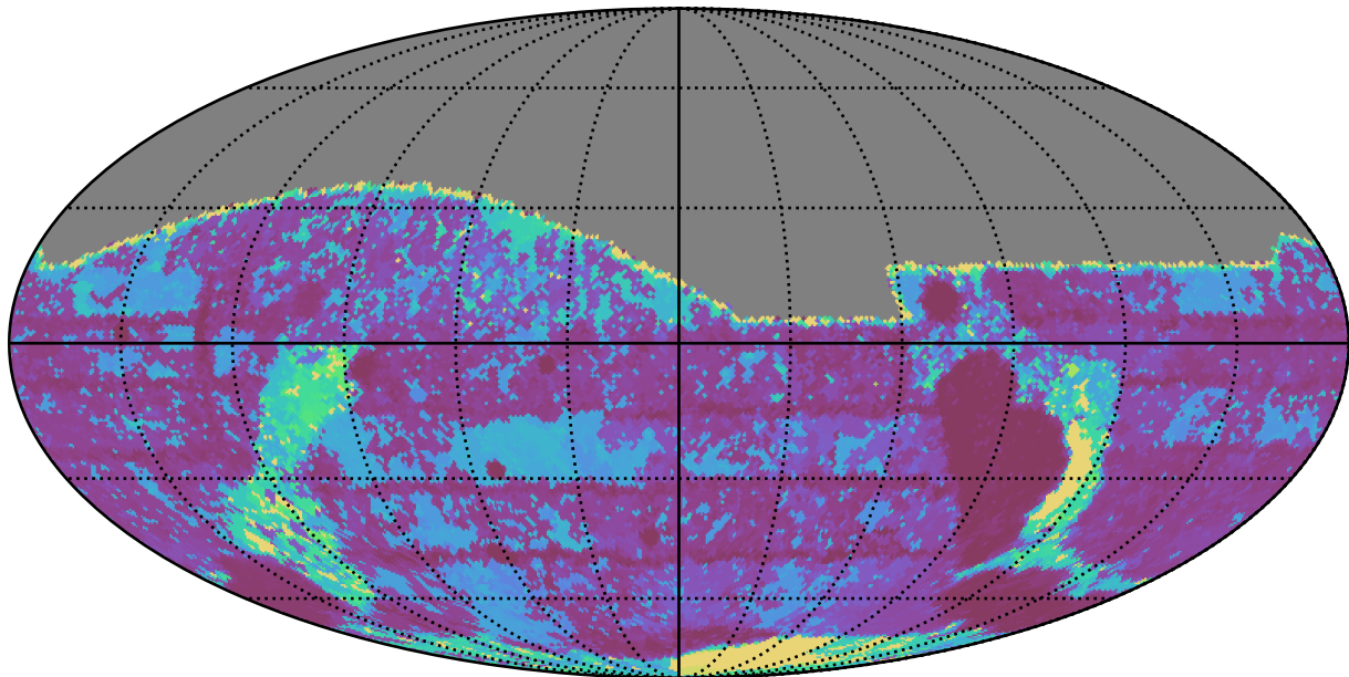
ddf_loaded_half_fl15_v3.4_10yrs All sky g band: Max Inter-Night Gap
