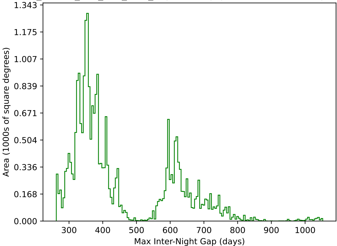
ddf_loaded_half_fl15_v3.4_10yrs All sky g band: Max Inter-Night Gap
