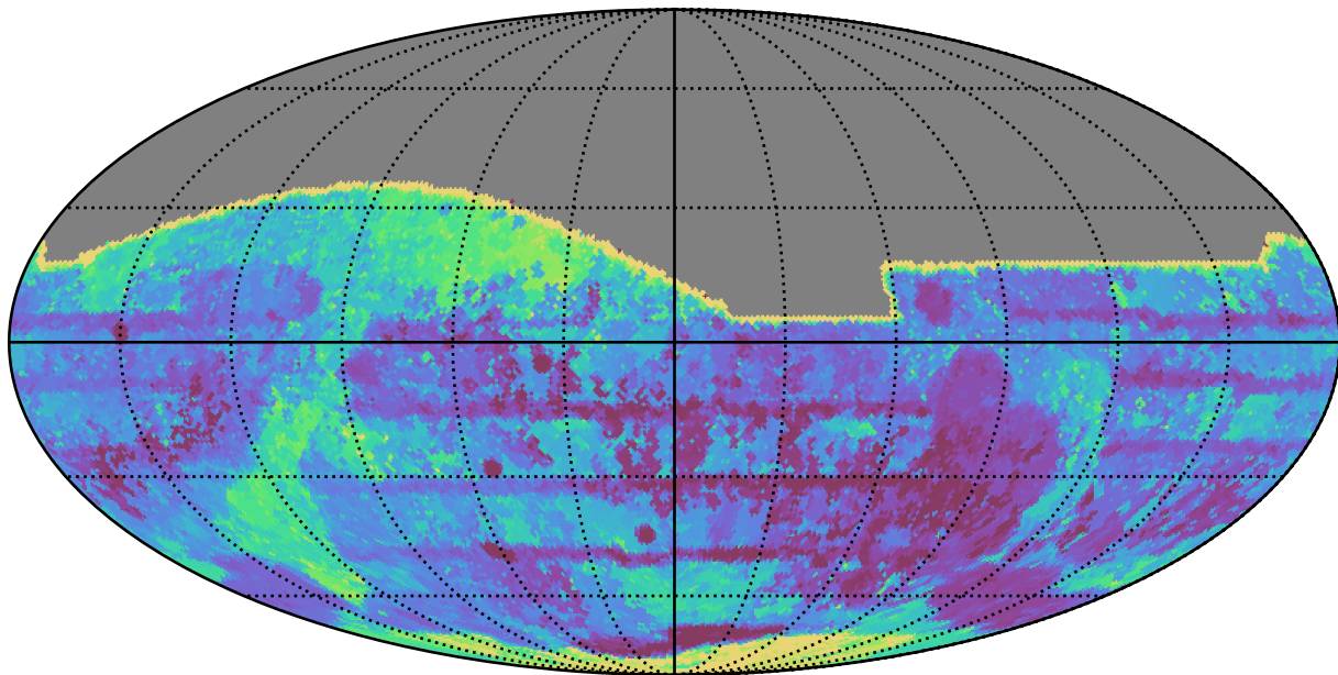
ddf_loaded_half_fl15_v3.4_10yrs All sky all bands: Max Inter-Night Gap
