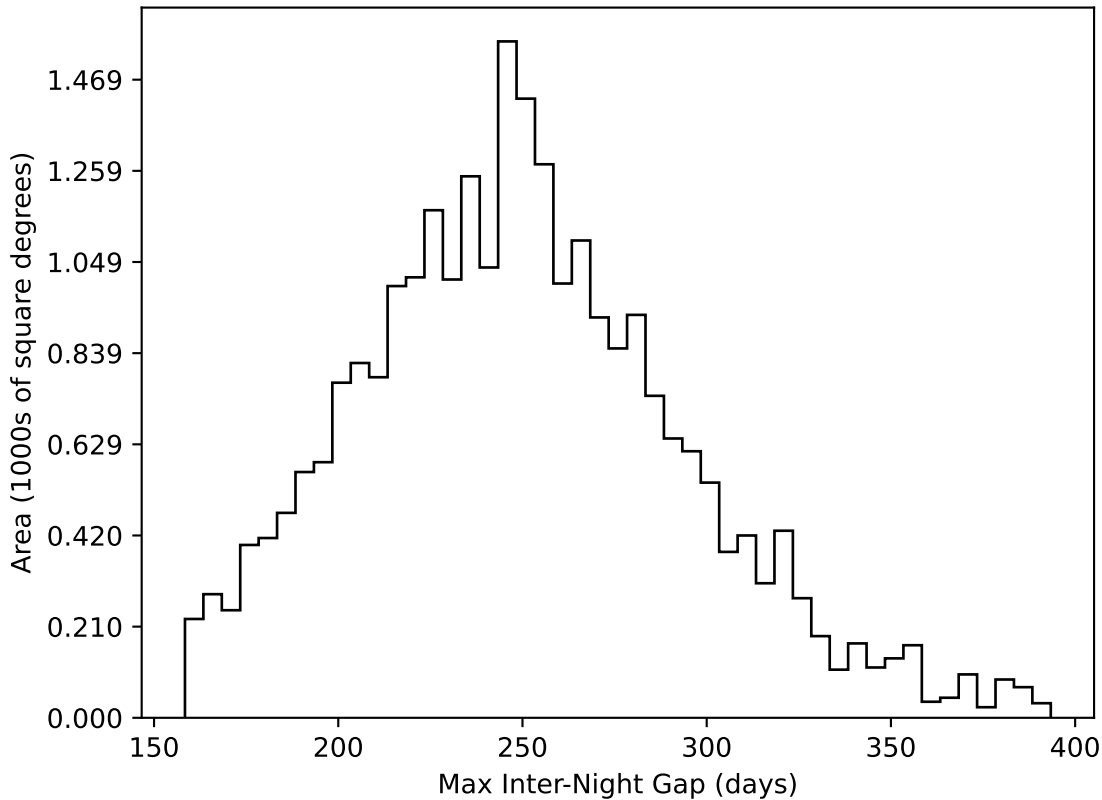
ddf_loaded_half_fl15_v3.4_10yrs All sky all bands: Max Inter-Night Gap
