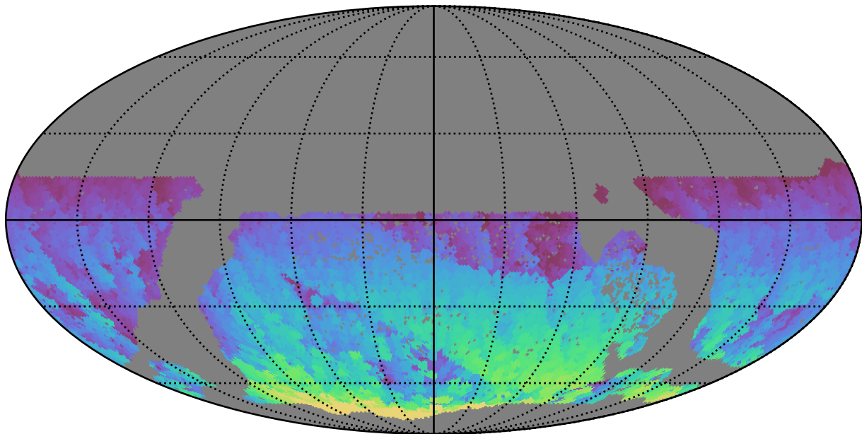
ddf_loaded_half_fl15_v3.4_10yrs WFD z band: Max HA
