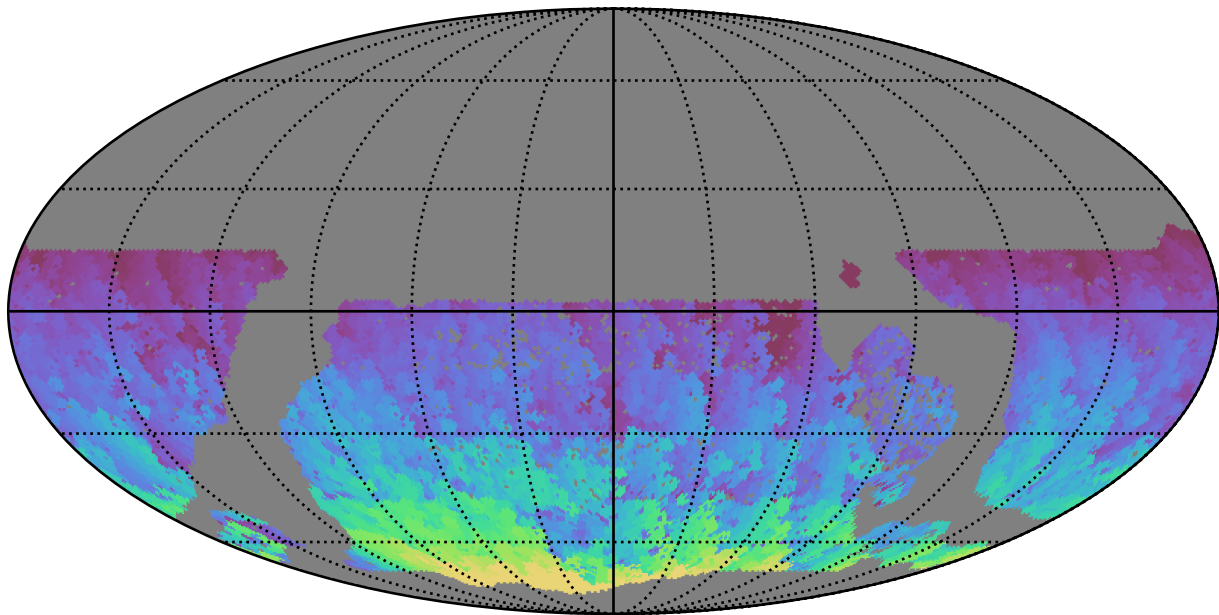
ddf_loaded_half_fl15_v3.4_10yrs WFD y band: Max HA
