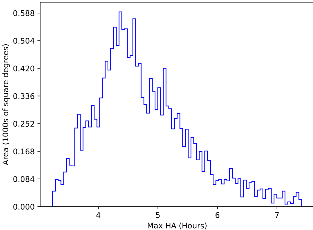
ddf_loaded_half_fl15_v3.4_10yrs WFD y band: Max HA
