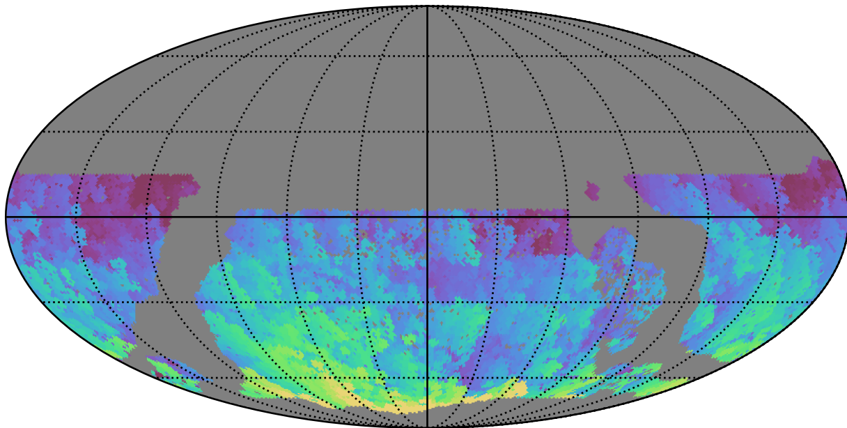
ddf_loaded_half_fl15_v3.4_10yrs WFD u band: Max HA
