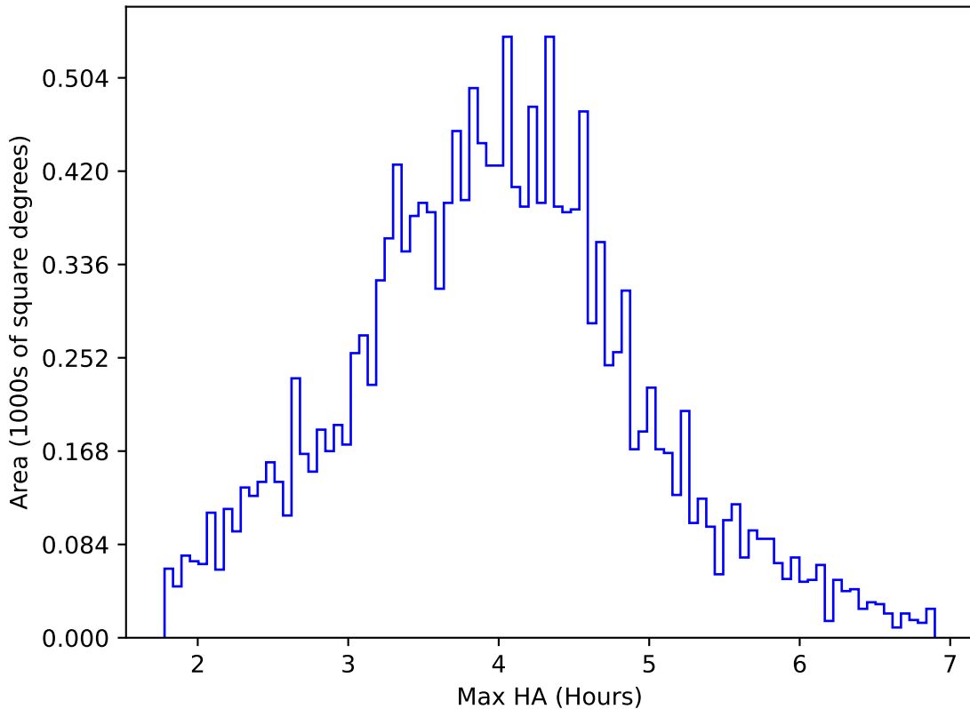
ddf_loaded_half_fl15_v3.4_10yrs WFD u band: Max HA
