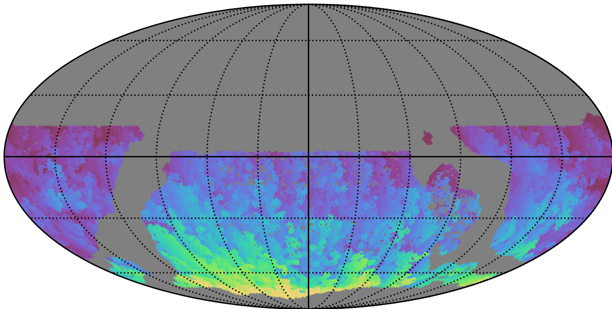
ddf_loaded_half_fl15_v3.4_10yrs WFD r band: Max HA
