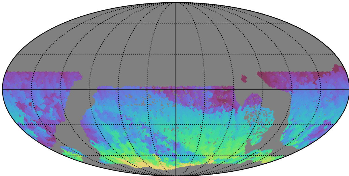
ddf_loaded_half_fl15_v3.4_10yrs WFD i band: Max HA
