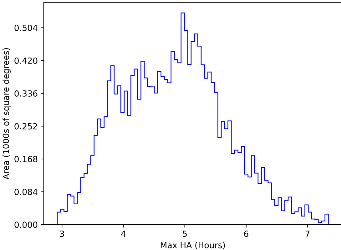
ddf_loaded_half_fl15_v3.4_10yrs WFD i band: Max HA
