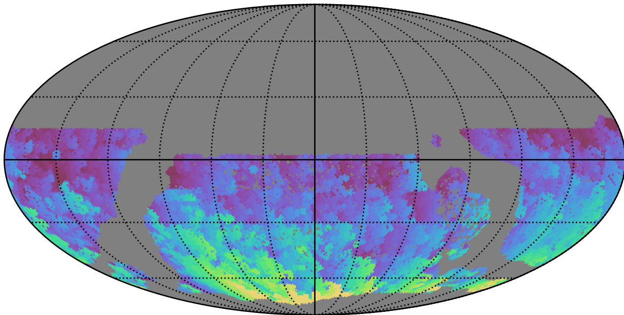
ddf_loaded_half_fl15_v3.4_10yrs WFD g band: Max HA
