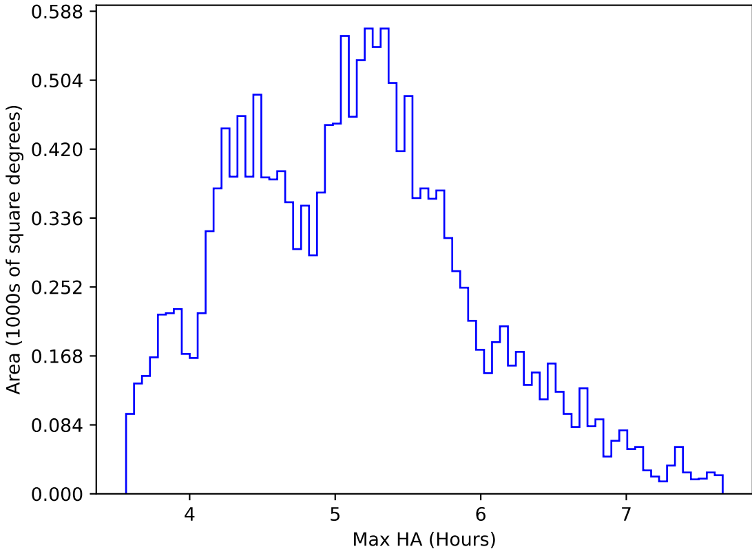
ddf_loaded_half_fl15_v3.4_10yrs WFD all bands: Max HA
