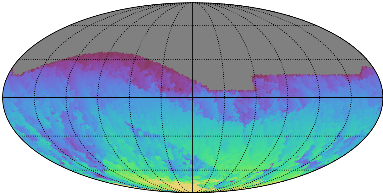
ddf_loaded_half_fl15_v3.4_10yrs All sky z band: Max HA
