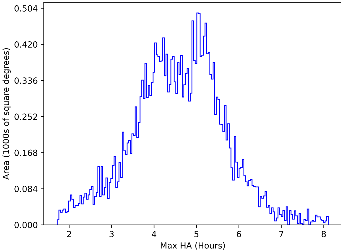
ddf_loaded_half_fl15_v3.4_10yrs All sky z band: Max HA
