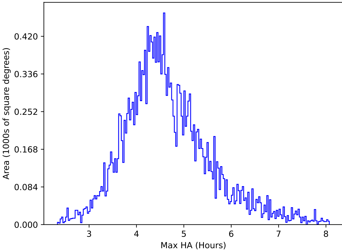
ddf_loaded_half_fl15_v3.4_10yrs All sky y band: Max HA
