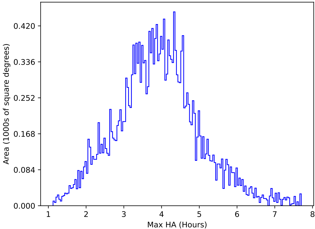
ddf_loaded_half_fl15_v3.4_10yrs All sky u band: Max HA
