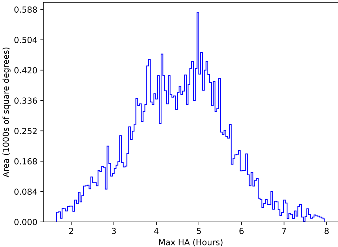
ddf_loaded_half_fl15_v3.4_10yrs All sky i band: Max HA
