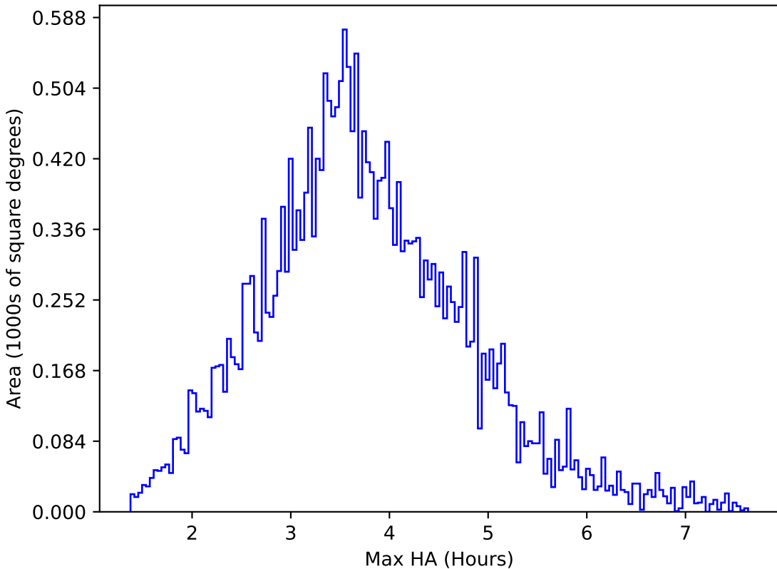
ddf_loaded_half_fl15_v3.4_10yrs All sky g band: Max HA
