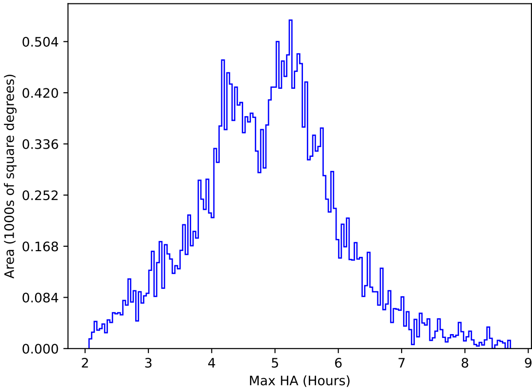
ddf_loaded_half_fl15_v3.4_10yrs All sky all bands: Max HA
