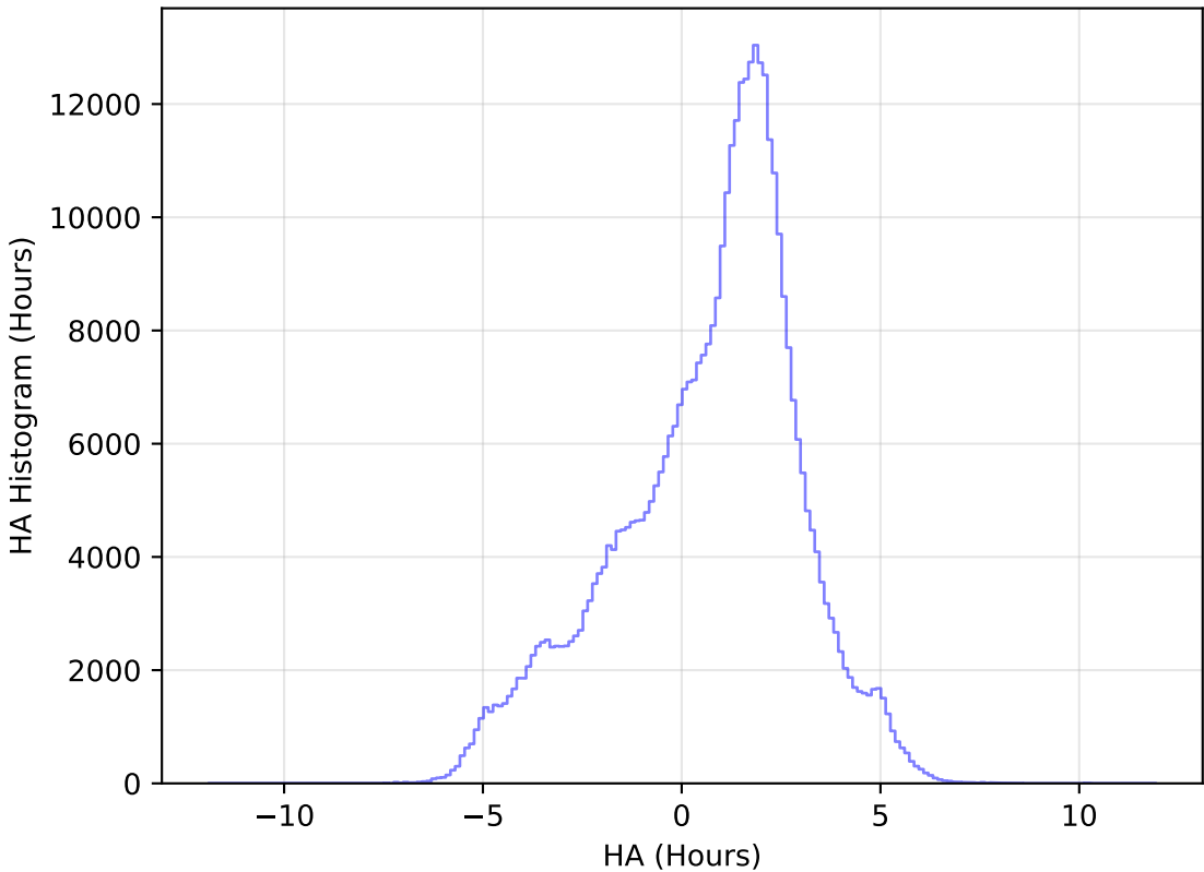
ddf_loaded_half_fl15_v3.4_10yrs WFD z band: HA Histogram
