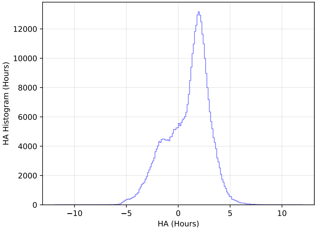
ddf_loaded_half_fl15_v3.4_10yrs WFD y band: HA Histogram
