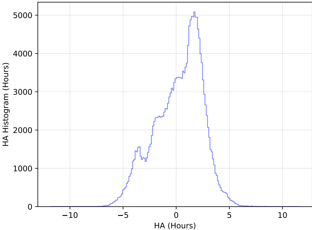
ddf_loaded_half_fl15_v3.4_10yrs WFD g band: HA Histogram
