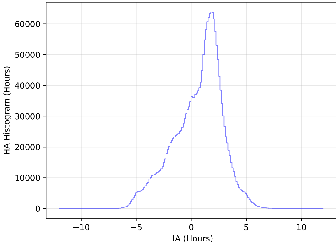
ddf_loaded_half_fl15_v3.4_10yrs WFD all bands: HA Histogram
