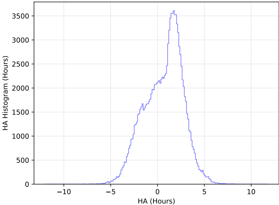
ddf_loaded_half_fl15_v3.4_10yrs All sky u band: HA Histogram
