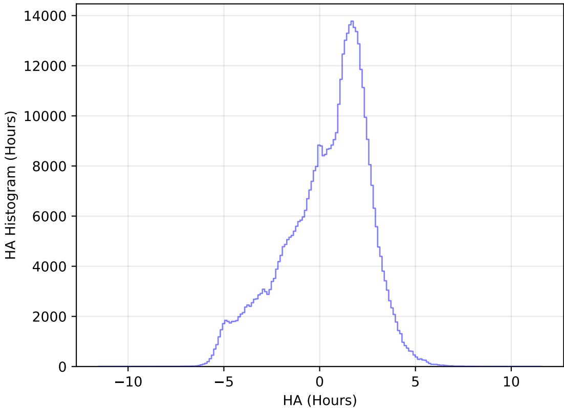
ddf_loaded_half_fl15_v3.4_10yrs All sky r band: HA Histogram
