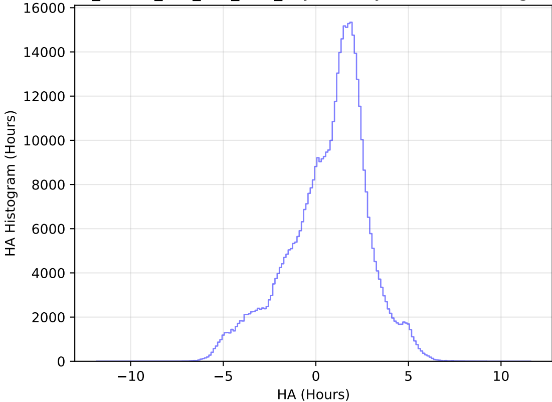
ddf_loaded_half_fl15_v3.4_10yrs All sky i band: HA Histogram
