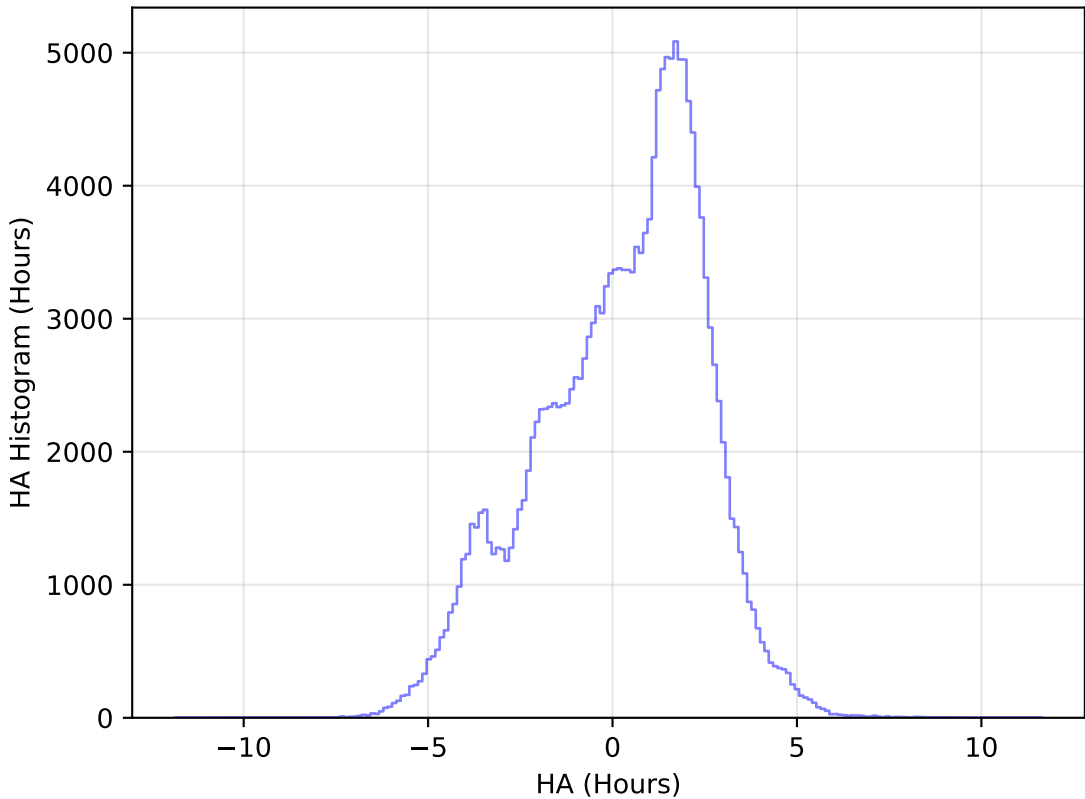
ddf_loaded_half_fl15_v3.4_10yrs All sky g band: HA Histogram
