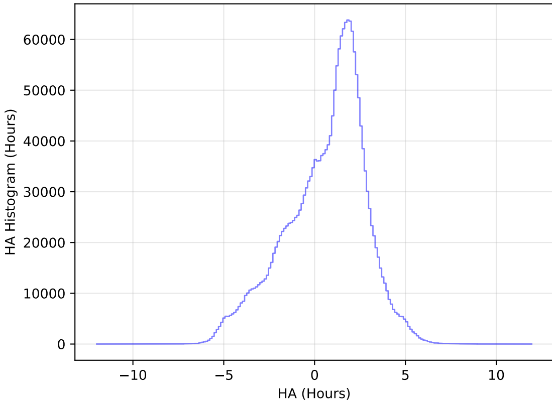
ddf_loaded_half_fl15_v3.4_10yrs All sky all bands: HA Histogram
