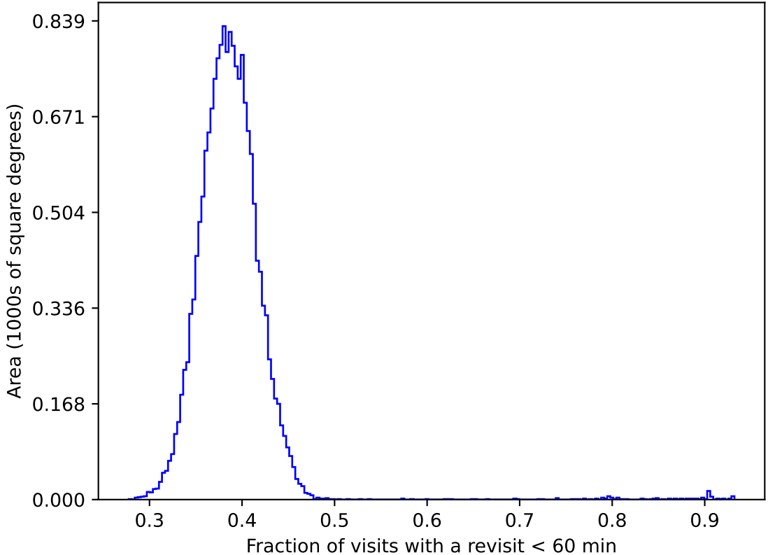
ddf_loaded_half_fl15_v3.4_10yrs gri WFD: Fraction of visits with a revisit < 60 min
