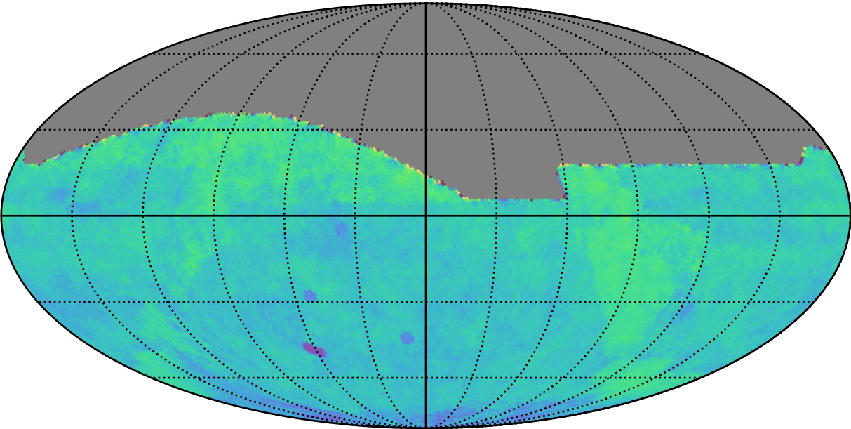
ddf_loaded_half_fl15_v3.4_10yrs gri All sky: Fraction of visits in pairs (10-60 min)
