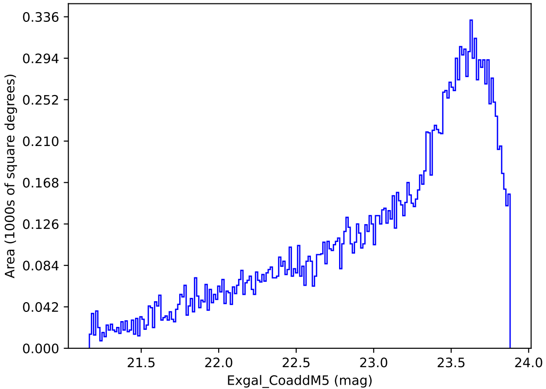
ddf_loaded_half_fl15_v3.4_10yrs Yr 3-4 y band: Exgal_CoaddM5
