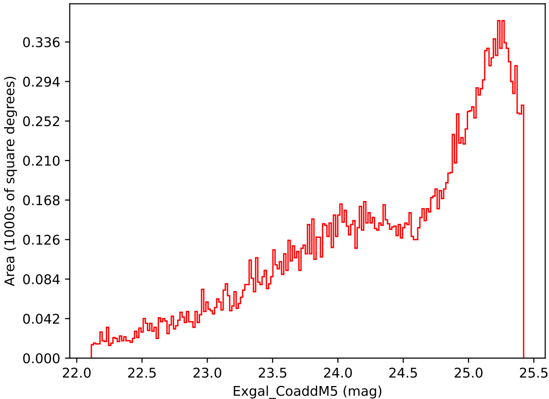
ddf_loaded_half_fl15_v3.4_10yrs Yr 3-4 i band: Exgal_CoaddM5
