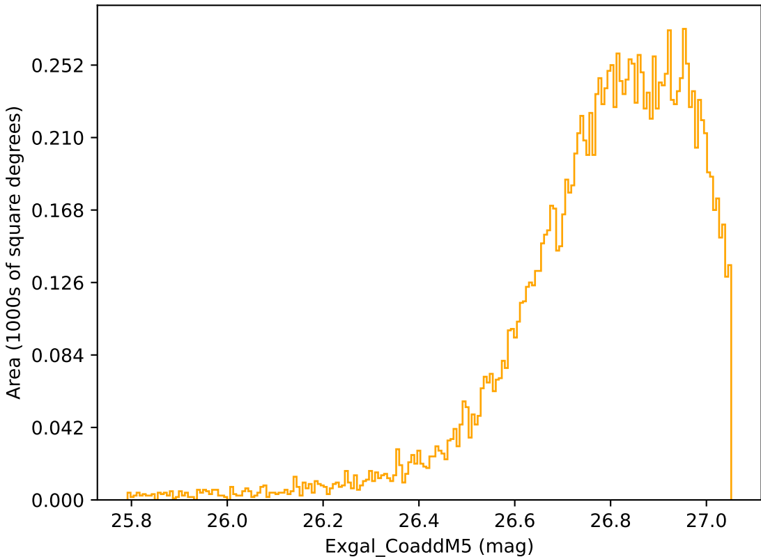
ddf_loaded_half_fl15_v3.4_10yrs WFD r band: Exgal_CoaddM5
