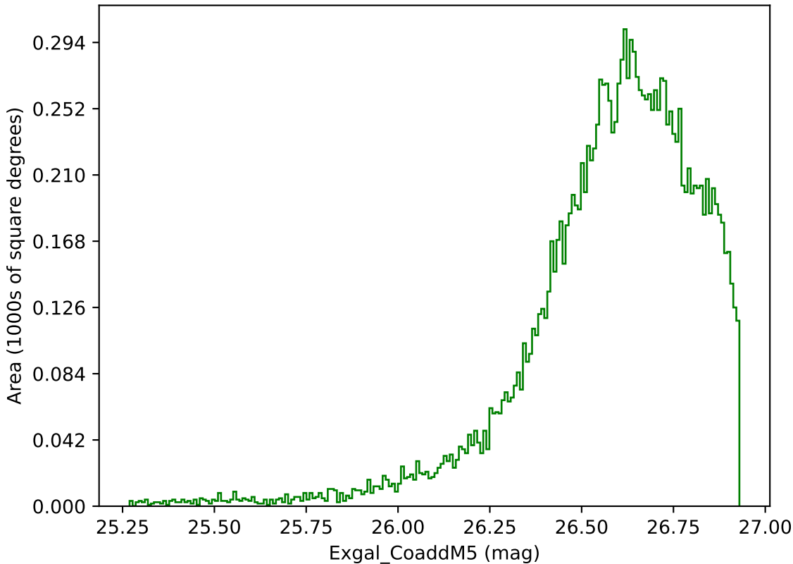
ddf_loaded_half_fl15_v3.4_10yrs WFD g band: Exgal_CoaddM5
