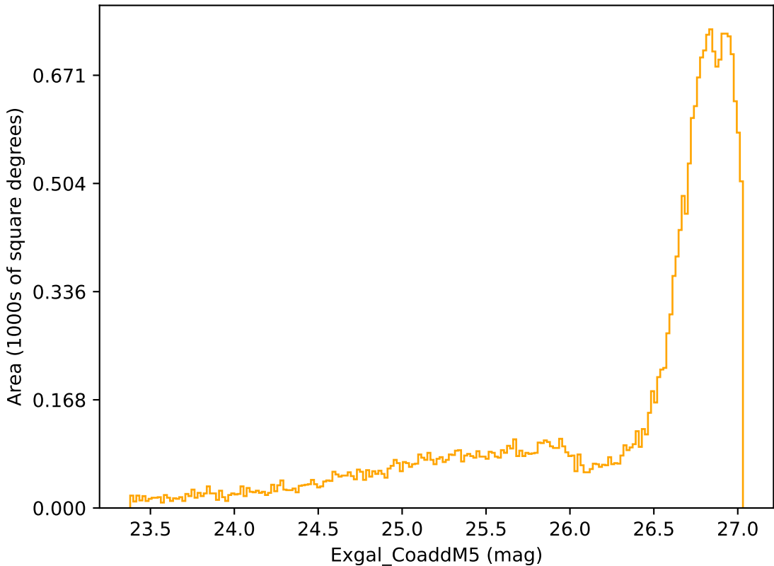
ddf_loaded_half_fl15_v3.4_10yrs All sky r band: Exgal_CoaddM5
