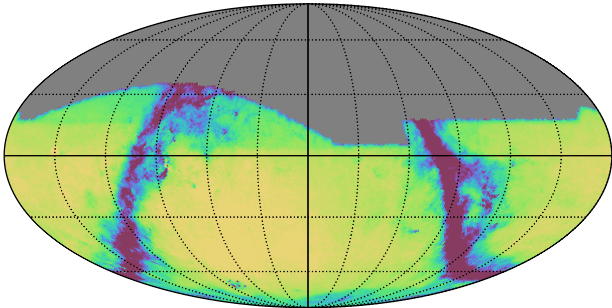
ddf_loaded_half_fl15_v3.4_10yrs All sky g band: Exgal_CoaddM5
