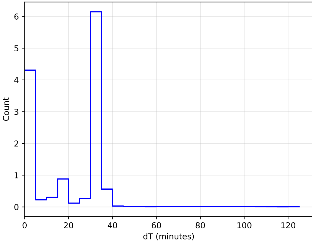
ddf_loaded_half_fl15_v3.4_10yrs All sky: DeltaT Histogram 1e6
