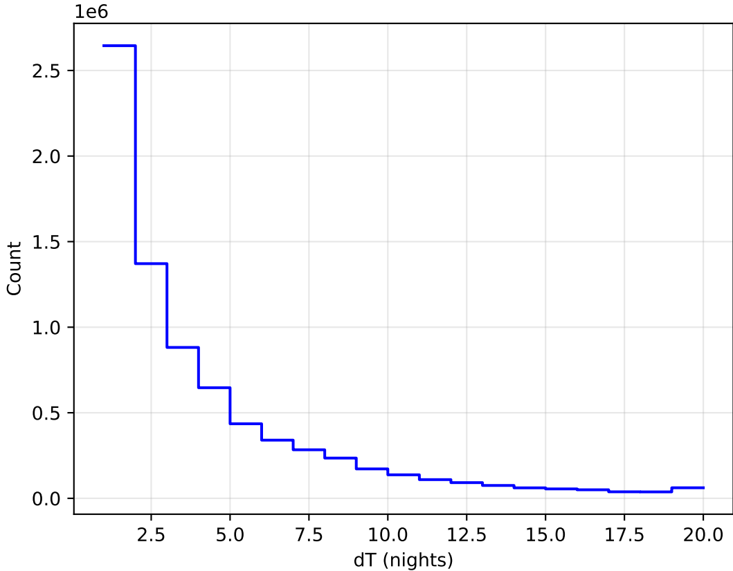
ddf_loaded_half_fl15_v3.4_10yrs WFD all bands: DeltaNight Histogram
