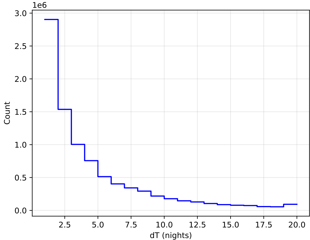
ddf_loaded_half_fl15_v3.4_10yrs All sky all bands: DeltaNight Histogram
