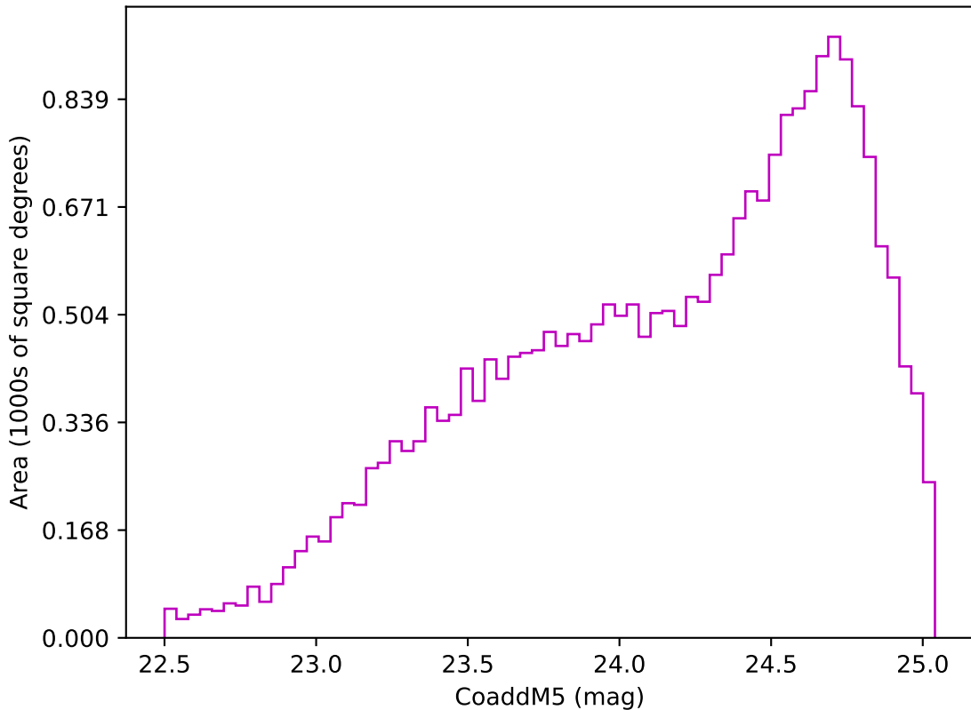
ddf_loaded_half_fl15_v3.4_10yrs Yr 3-4 z band: CoaddM5
