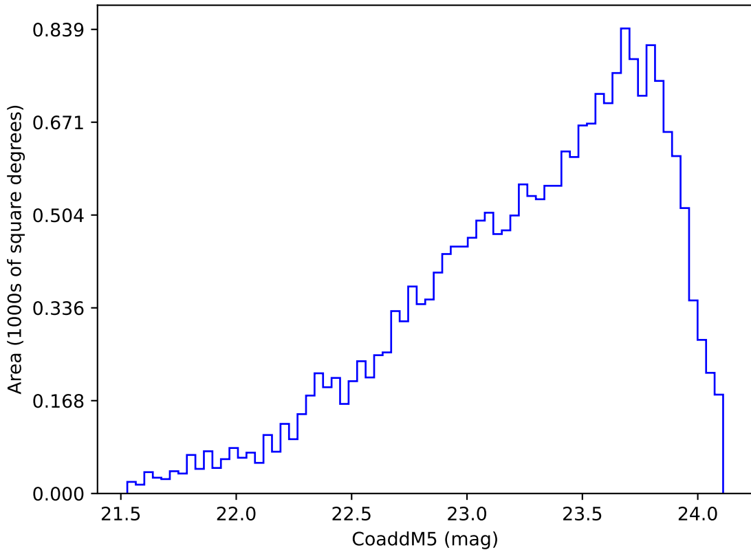
ddf_loaded_half_fl15_v3.4_10yrs Yr 3-4 y band: CoaddM5
