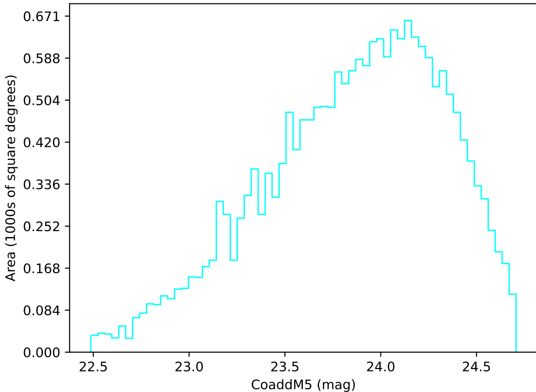
ddf_loaded_half_fl15_v3.4_10yrs Yr 3-4 u band: CoaddM5
