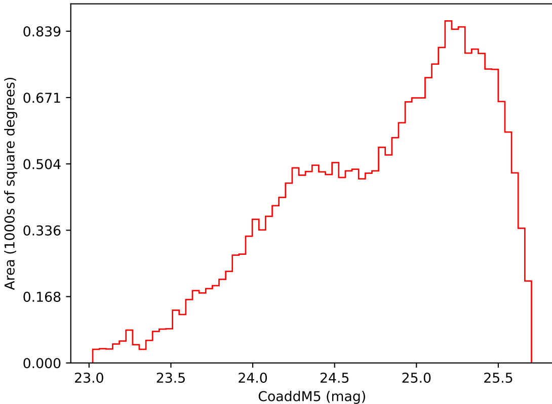
ddf_loaded_half_fl15_v3.4_10yrs Yr 3-4 i band: CoaddM5
