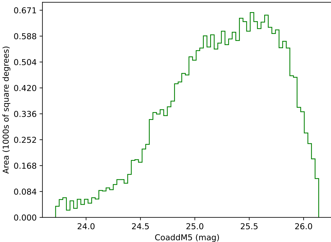
ddf_loaded_half_fl15_v3.4_10yrs Yr 3-4 g band: CoaddM5
