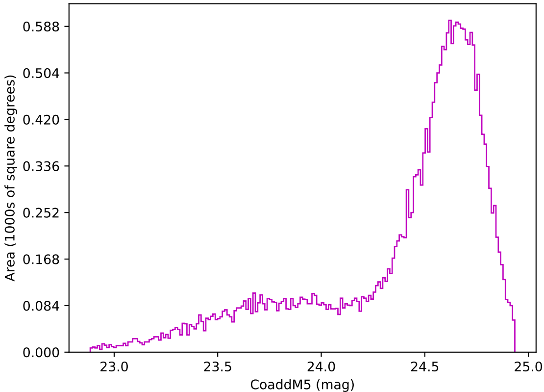
ddf_loaded_half_fl15_v3.4_10yrs Yr 1 z band: CoaddM5
