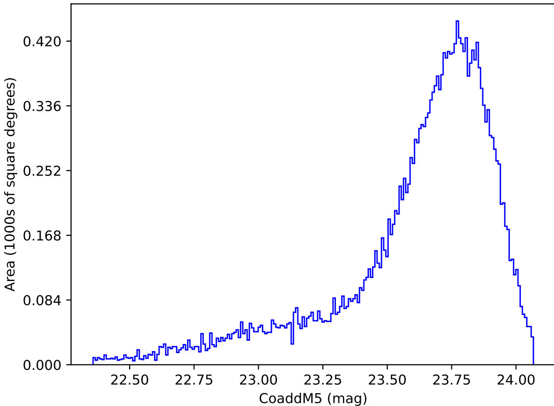
ddf_loaded_half_fl15_v3.4_10yrs Yr 1 y band: CoaddM5
