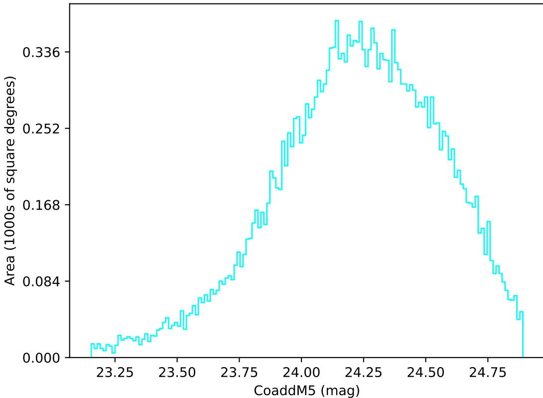
ddf_loaded_half_fl15_v3.4_10yrs Yr 1 u band: CoaddM5
